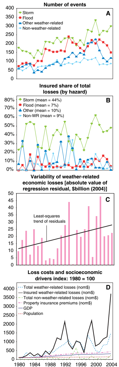
Fig. 2. (A to D) Trends in (A) global numbers of weather-related events, (B) insured share, (C) variability of total losses, and (D) economic impacts and demographic drivers. Insured and total property losses ($45 billion and $107 billion in 2004, respectively) are rising faster than premiums, population, or economic growth. Data exclude health and life insurance premiums and losses. Non-inflation-adjusted economic data are shown in relation to GDP. Inflation-adjusted economic losses from catastrophic events rose by 8-fold between the 1960s and 1990s and insured losses by 17-fold (17). [Sources: Natural hazard statistics and losses from Munich Re, NatCatSERVICE; Premiums from Swiss Re, Sigma ]
